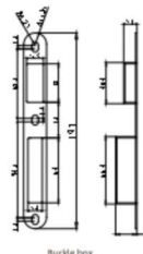
Buckle box
